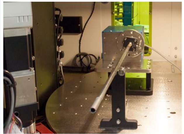
Laser Marking Site with Custom Rotating Tooling
